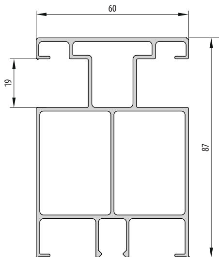
PG10 CleverBox
