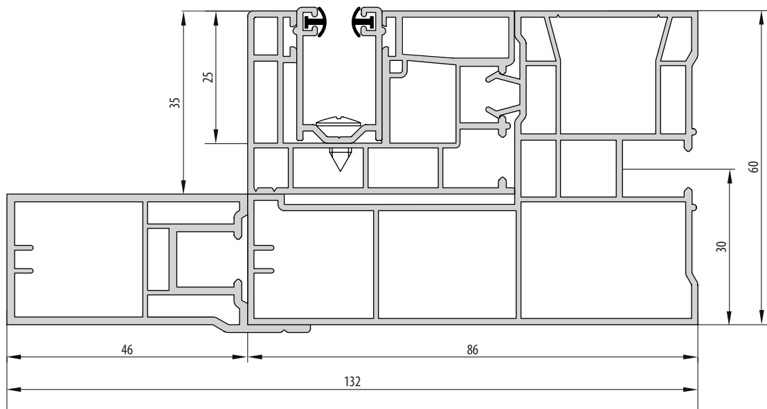
5080 - 5081 Elite XT
